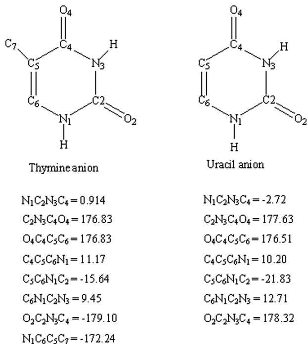
Figure 2. Torsional angle values (in degrees) for thymine and uracil at the optimised geometries. The same torsional angles for neutral system are equal to 180° or 0°.
